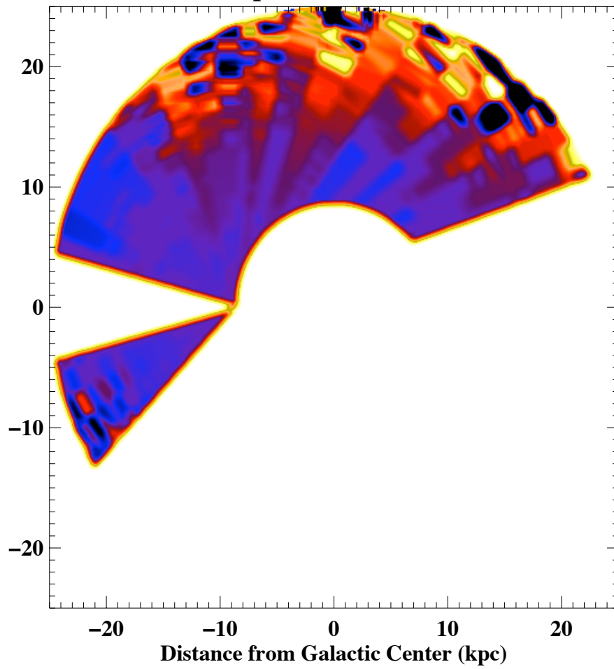
The Warp of the Galactic Plane
