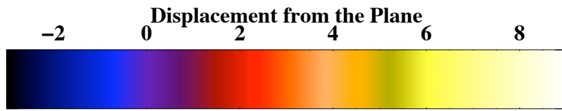
The Warp of the Galactic Plane
